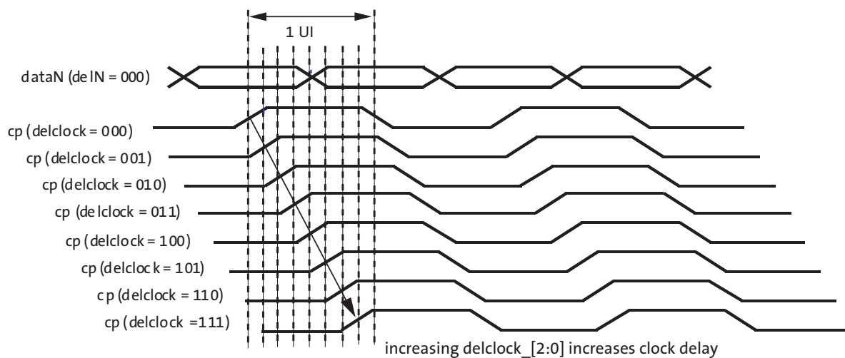
Figure 24: Delaying the clock_lane with Respect to data_lane
