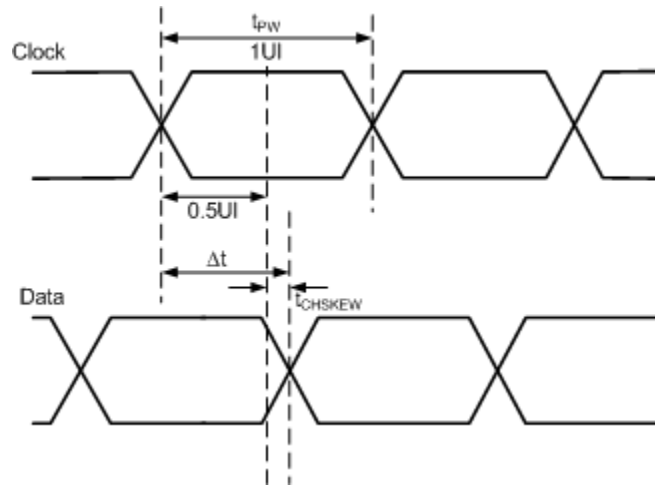
Figure 12: Clock-to-Data Skew Timing Diagram
