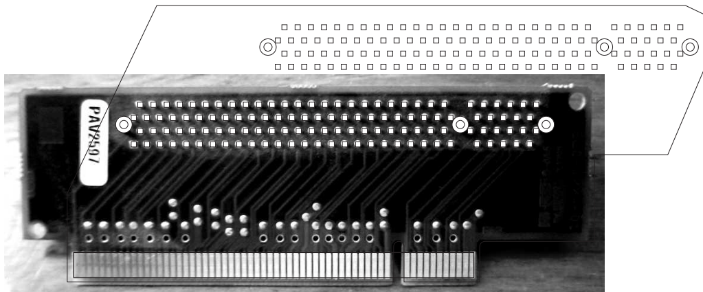
TAM TwinSlot PCI Riser
