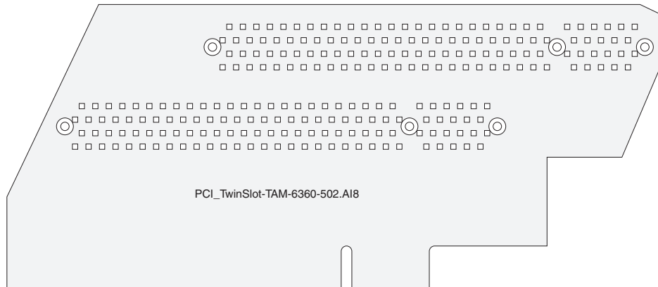
TAM TwinSlot PCI Riser
