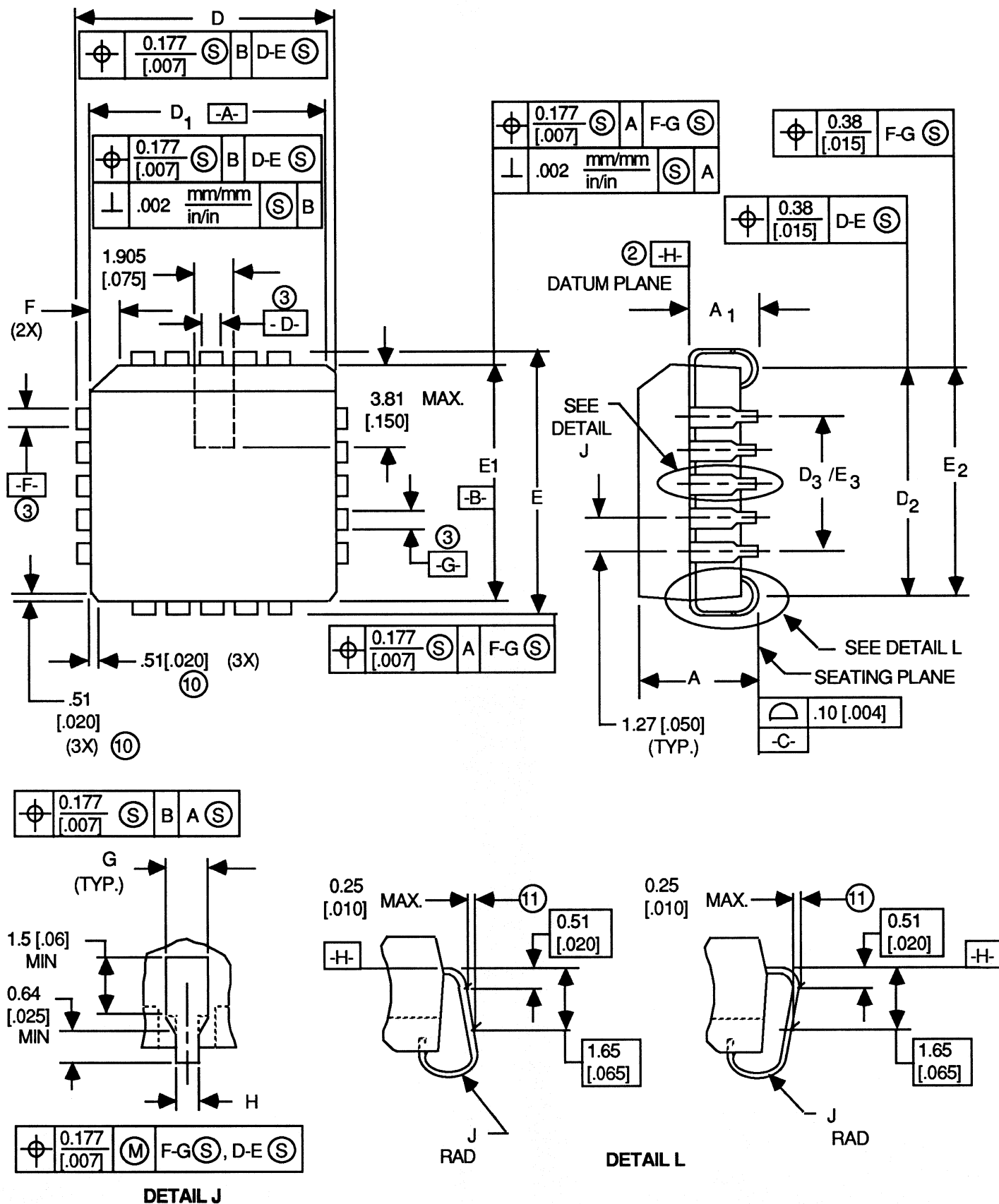
FIGURE 3. DIMENSIONS
