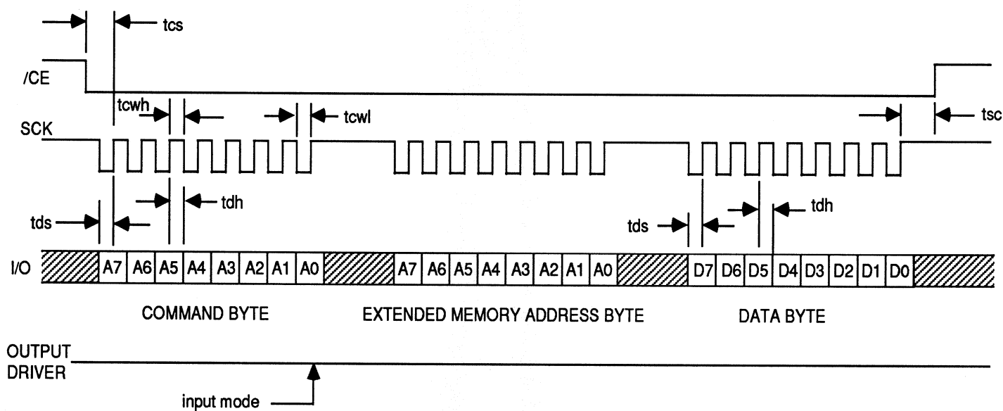
FIGURE 7. EXTENDED WRITE TIMING
