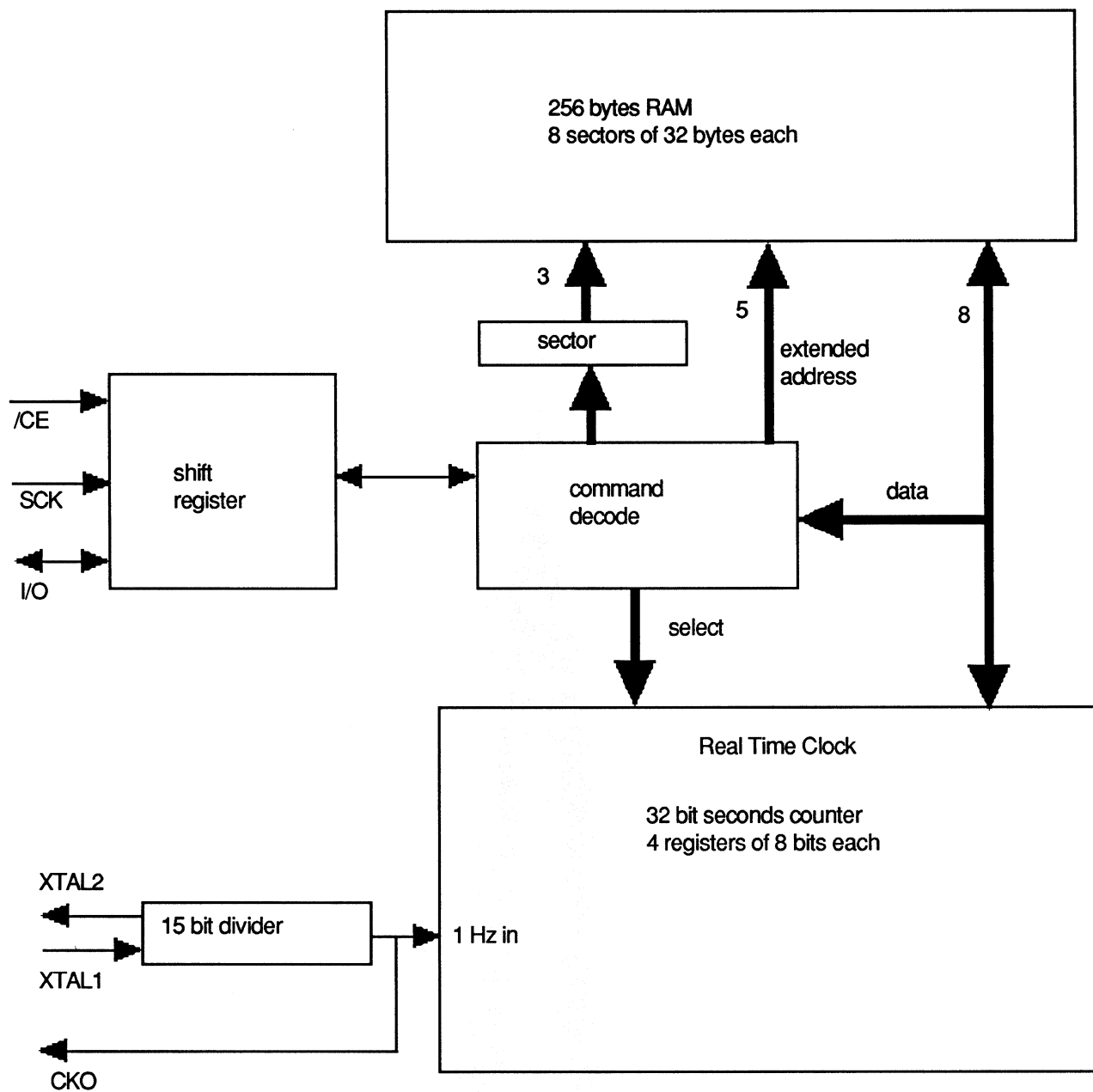
FIGURE 2. BLOCK DIAGRAM
