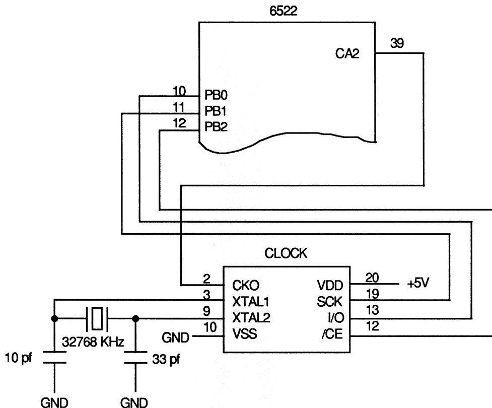
FIGURE 11. CLOCK CONNECTIONS IN MAC
