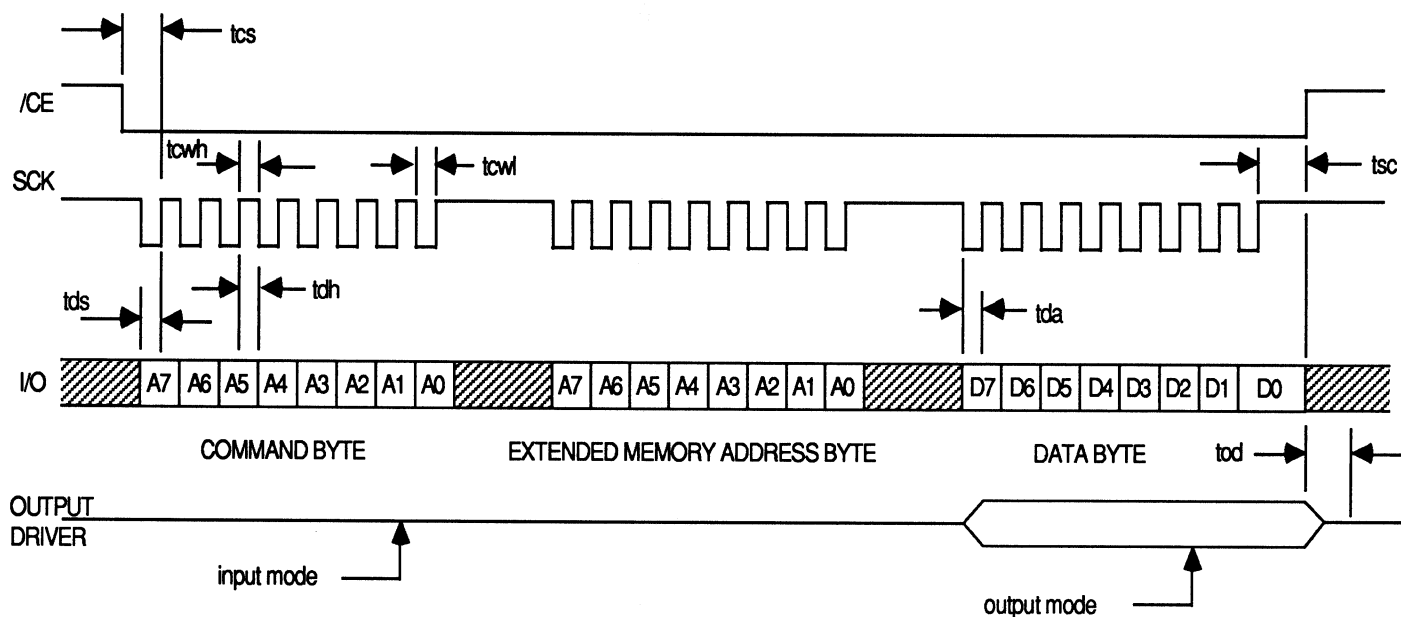
FIGURE 6. EXTENDED READ TIMING
